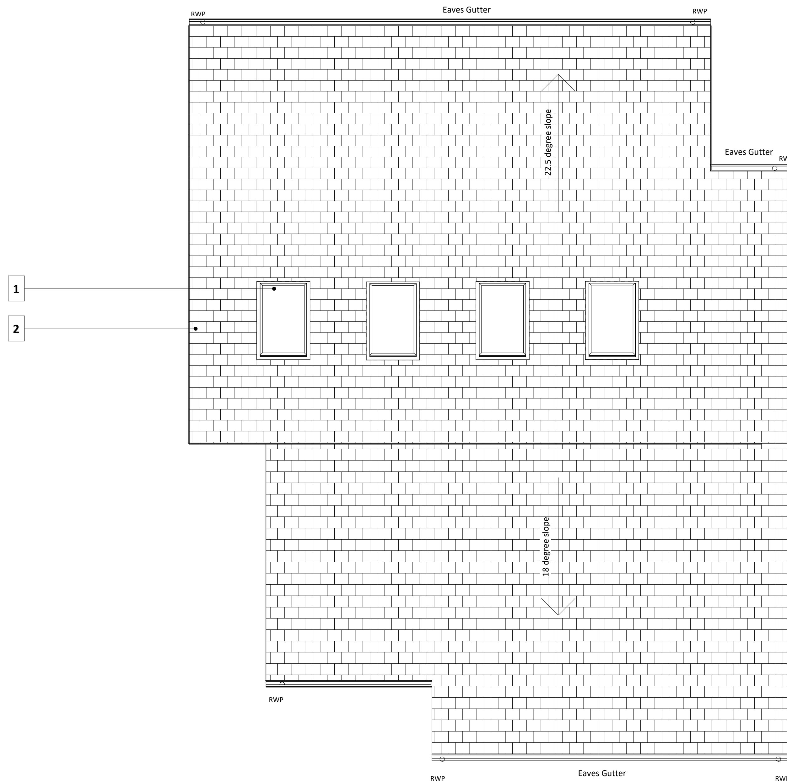
1. Proposed Roof Plan SCALE - 1 : 50@A1
