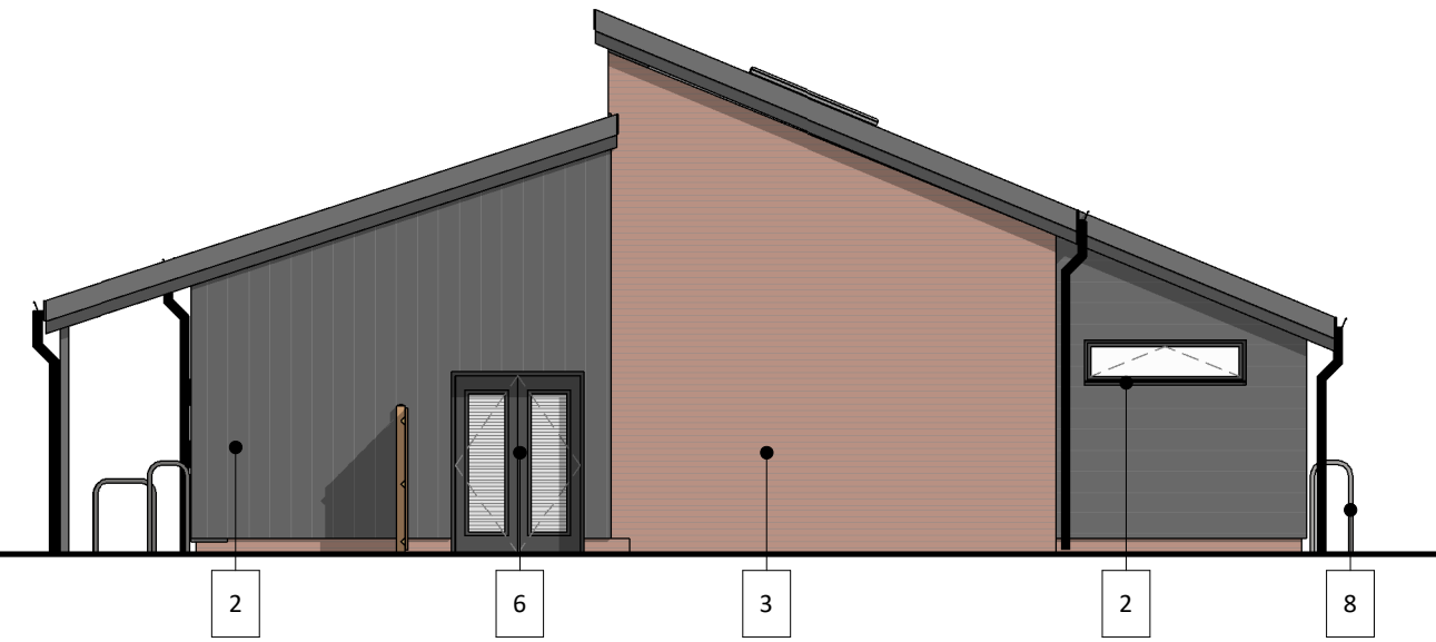
4. Proposed South Elevation SCALE - 1 : 100@A3
