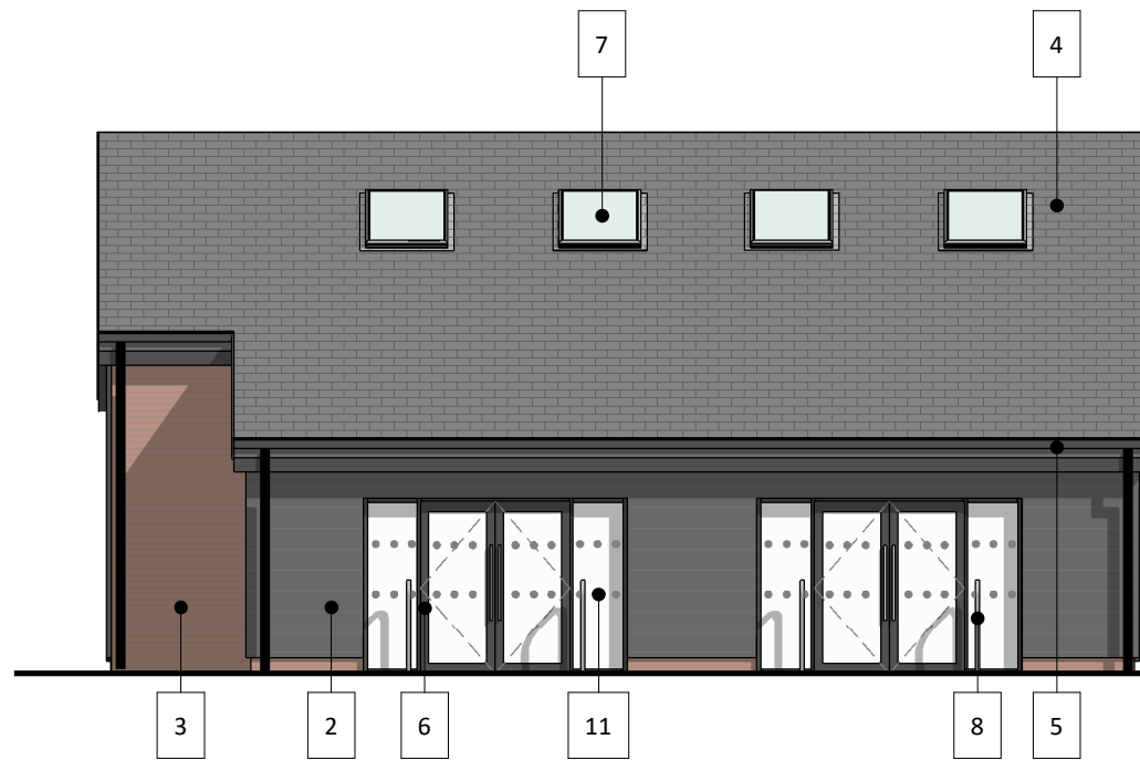
1. Proposed West Elevation SCALE - 1 : 100@A3
