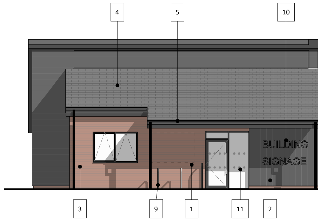
1. Proposed West Elevation SCALE - 1 : 100@A3
