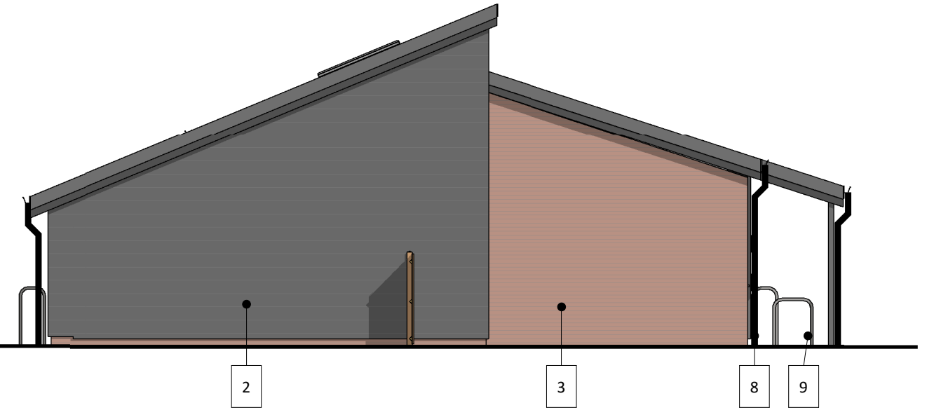
2. Proposed North Elevation SCALE - 1 : 100@A3
