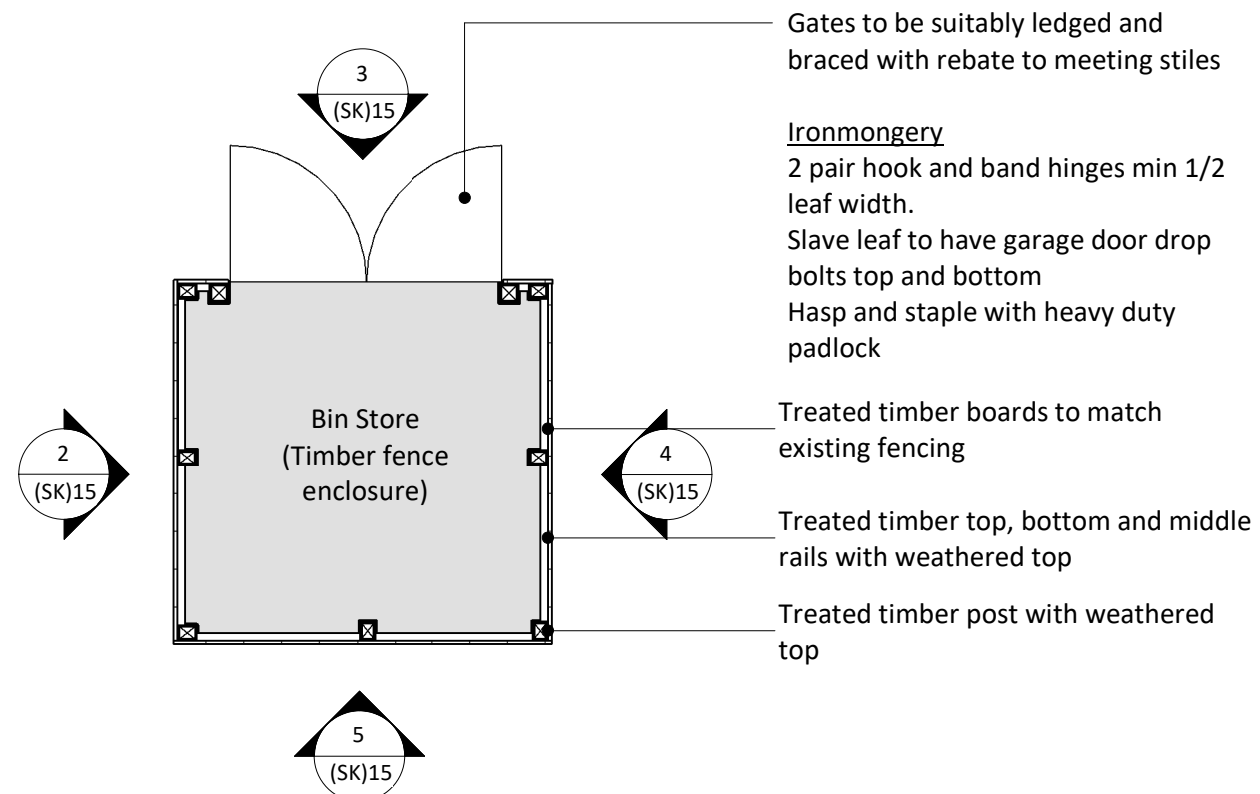
1. Bin Store Enclosure Plan SCALE - 1 : 50@A3
