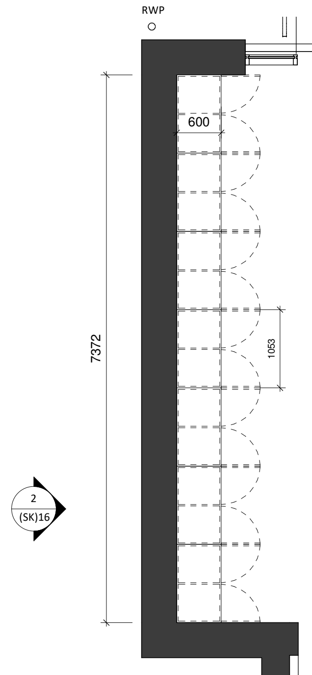
2. Fixed Hall Storage Plan SCALE - 1 : 50@A3
