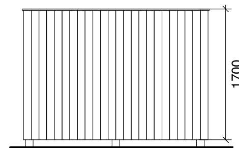
2. Bin Store Elevation 01 SCALE - 1 : 50@A3
