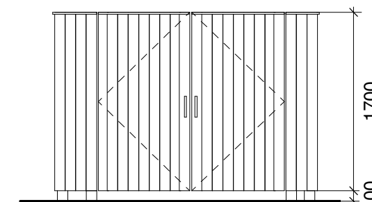
3. Bin Store Elevation 02 SCALE - 1 : 50@A3
