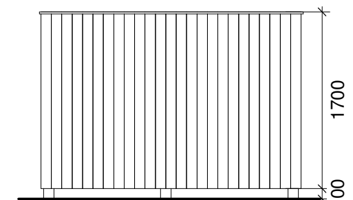
5. Bin Store Elevation 04 SCALE - 1 : 50@A3
